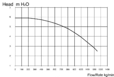
6-Meter-Pressure Pump
